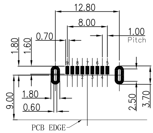
RECOMMENDED PCB LAYOUT TOLERANCES: ±0.05
