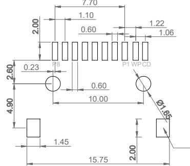
Recommended P.C.B Layout(Top Side)
